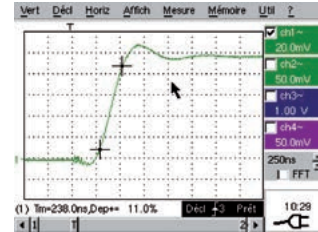
Pulse response
